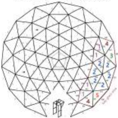
5m Dome Frame Layout (glass bay)
